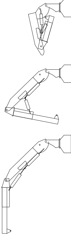
Crane Side View
